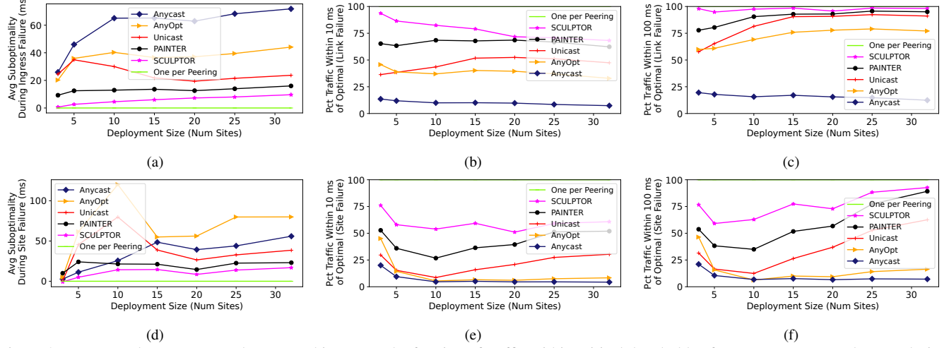
Figure 8: SCULPTOR lowers average latency and increases the fraction of traffic within critical thresholds of One-per-Peering latency during both link and site failures over many emulated deployments.
