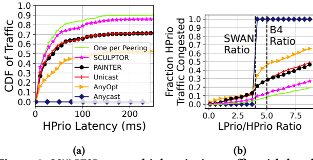
Figure 8: SCULPTOR routes high-priority traffic with low latency (8a) and minimal congestion from low-priority traffic (8b). We inferred LPrio/HPrio ratios for SWAN [19] and B4 [18] from those papers.
