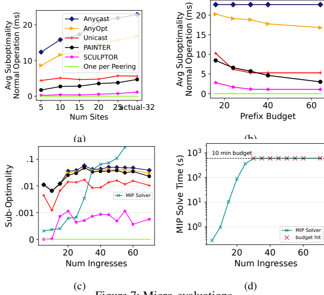
Figure 7: Micro-evaluations.
