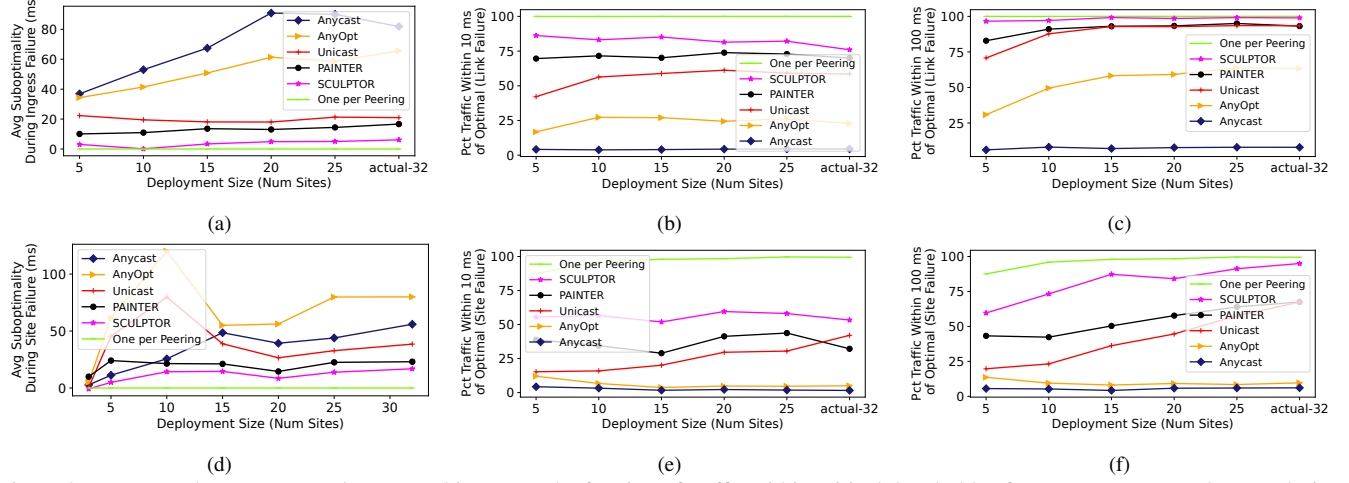
Figure 9: SCULPTOR lowers average latency and increases the fraction of traffic within critical thresholds of One-per-Peering latency during both link and site failures over many emulated deployments.
