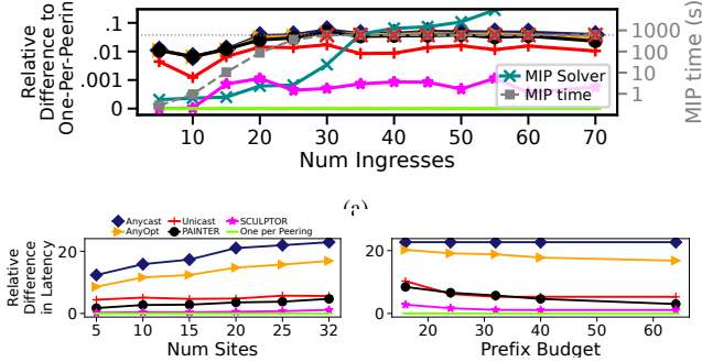
Figure 7: Micro-evaluations. (a) Sub-optimality of the latency+MLU objective relative to the one-per-peering bound as the deployment grows one ingress at a time (5 deployments per size; legend as in (b)) against the full advertisement MIP (HiGHS, 10-minute budget), whose solve time is the gray dashed line on the right axis; steady-state latency sub-optimality vs. number of sites (b) and prefix budget (c).
