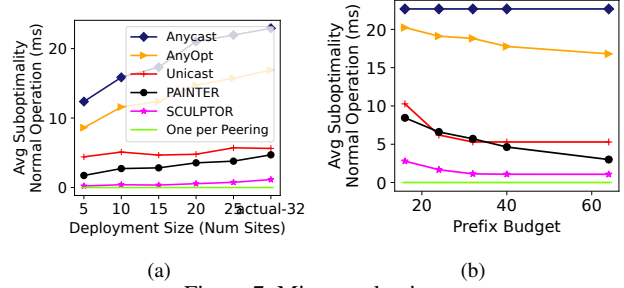
Figure 7: Micro evaluations.
