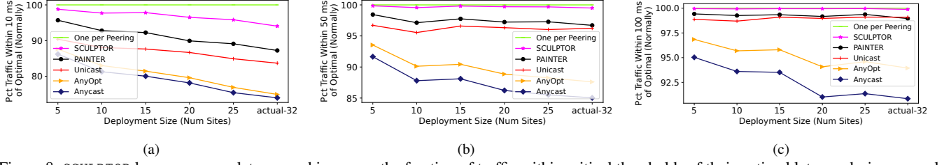
Figure 8: SCULPTOR lowers average latency and increases the fraction of traffic within critical thresholds of their optimal latency during normal operation.
