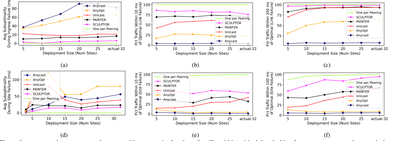
Figure 9: SCULPTOR lowers average latency and increases the fraction of traffic within critical thresholds of One-per-Peering latency during both link and site failures over many emulated deployments.
