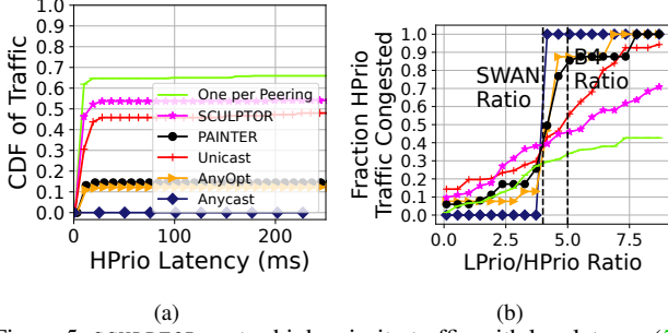
Figure 5: SCULPTOR routes high-priority traffic with low latency (5a) and minimal congestion from low-priority traffic (5b). We inferred LPrio/HPrio ratios for SWAN [19] and B4 [18] from those papers.
