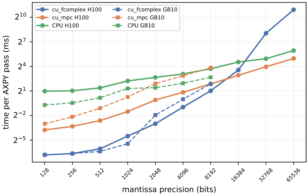
AXPY complex (MPC): solid=H100, dashed=GB10
