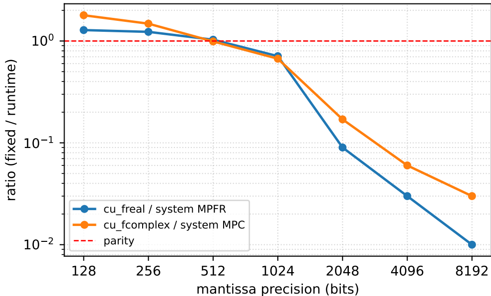
CPU only: fixed precision vs MPFR/MPC
