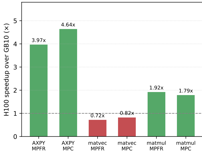
(b) H100 / GB10 GPU-time ratio
