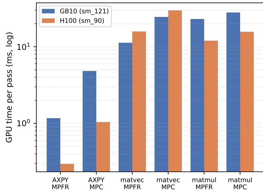
(a) GPU time: GB10 vs H100 (1024-bit)
