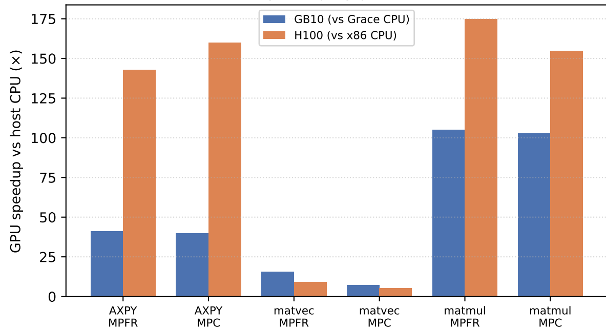
GPU-vs-CPU speedup by platform (1024-bit)
