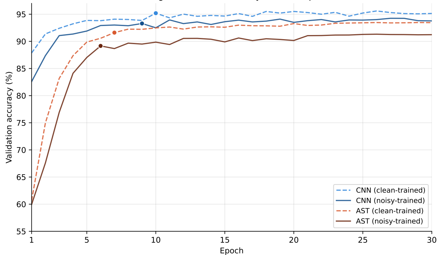
Training: validation accuracy over 30 epochs
