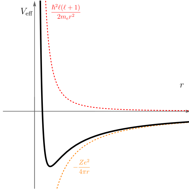
Figure 2: The effective potential for the electron in a hydrogen-like atom, including both the Coulomb potential and the centrifugal potential.
