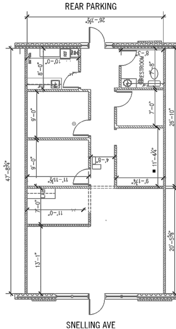
AS-BUILT
