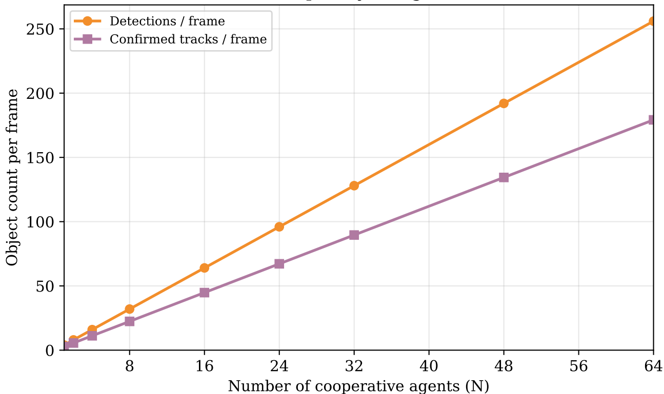
Scene Complexity vs Agent Count
