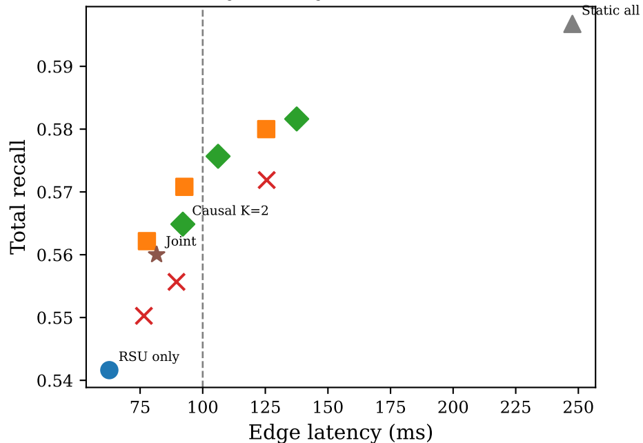
(a) Quality-latency tradeoff: total recall
