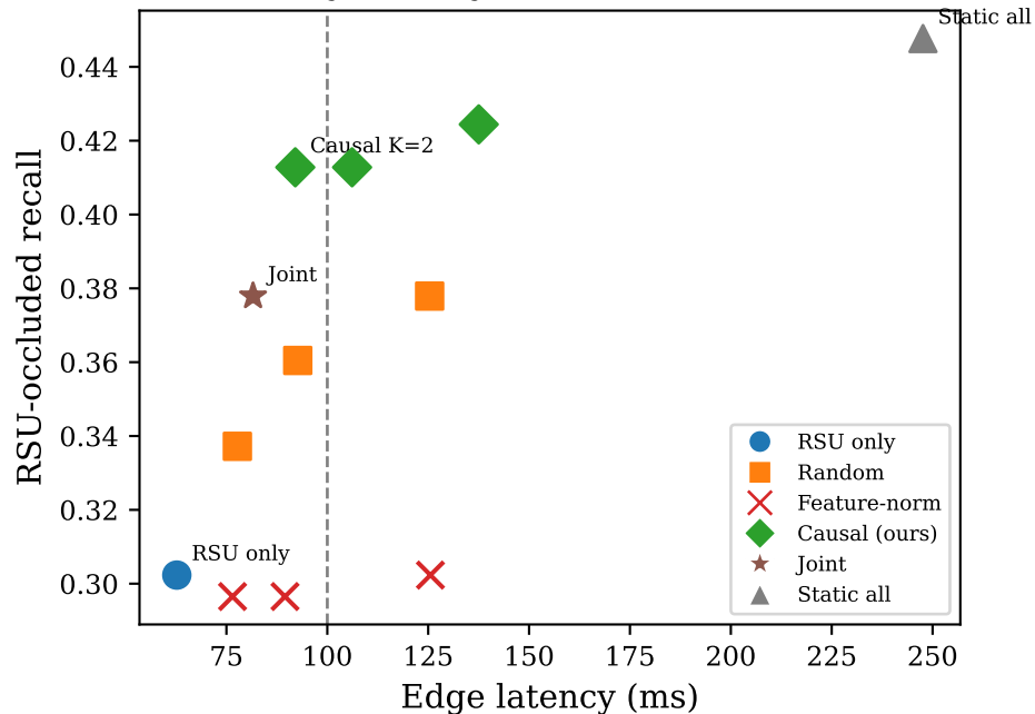
(b) Quality-latency tradeoff: occluded recall
