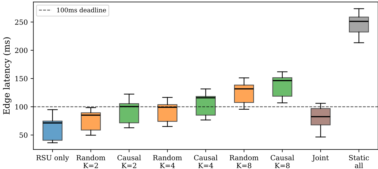
Per-tick latency distribution by selector and budget
