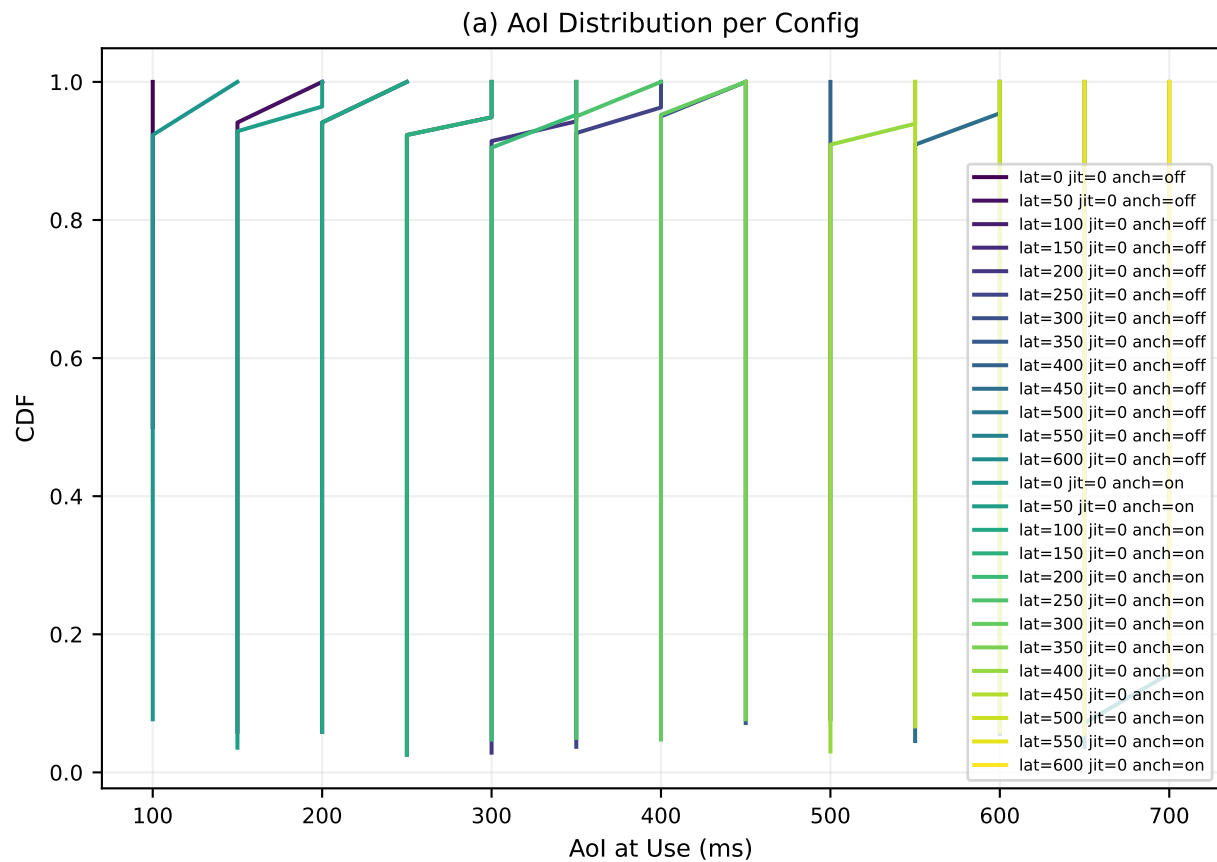
Fig 10: Age of Information at Brake Decision
