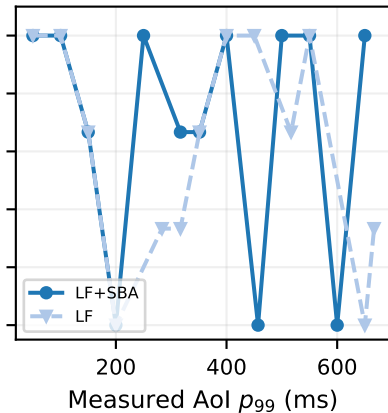
Late Fusion
