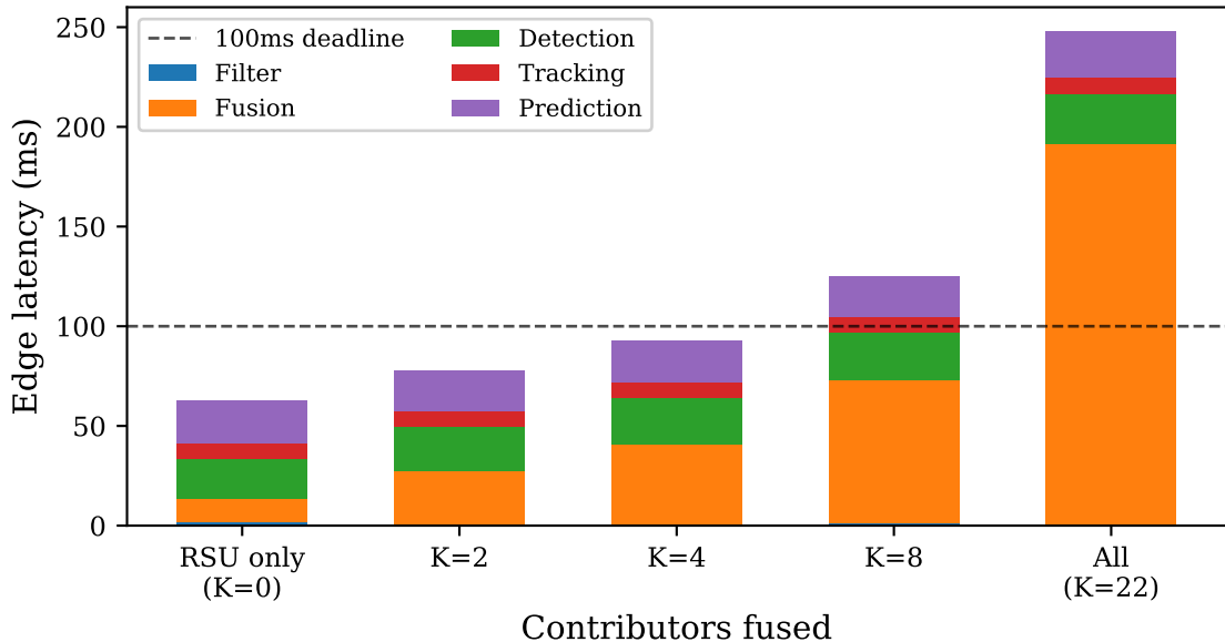
Per-stage latency scaling (rsu_250, N=23)
