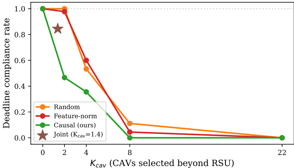
Fraction of ticks meeting 100ms deadline
