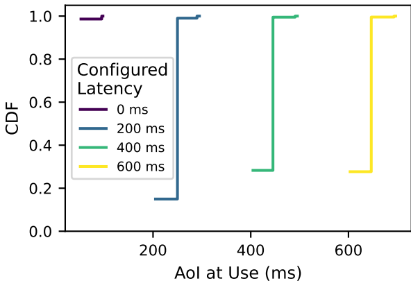
Aol Distribution
