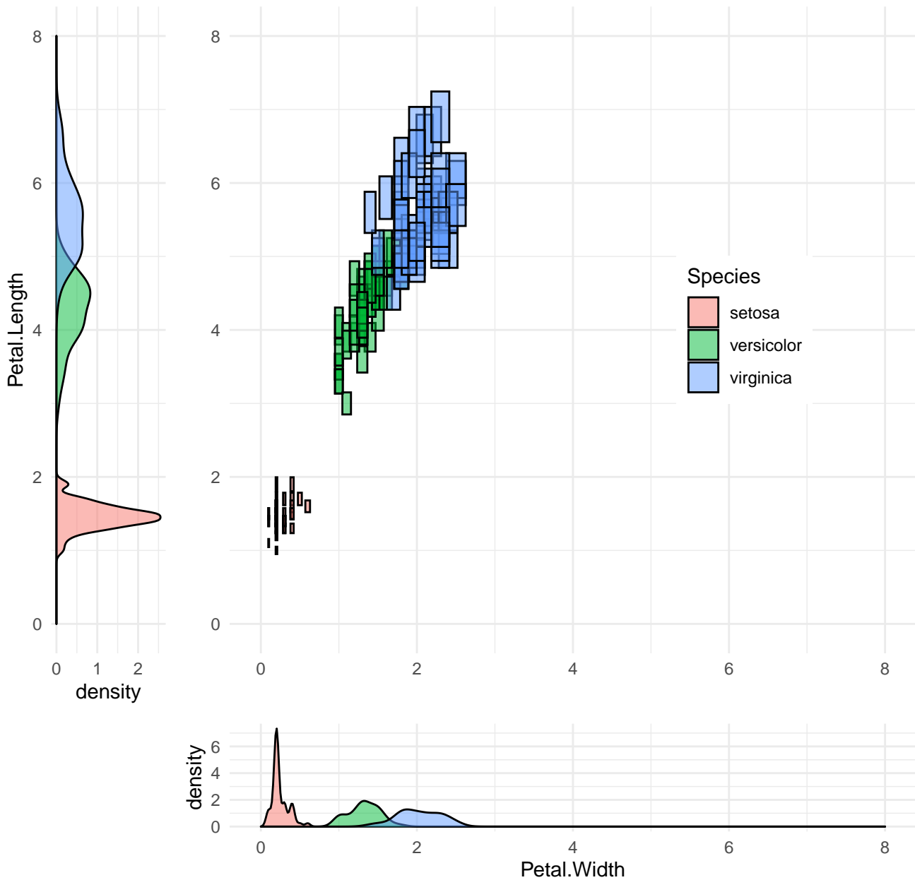
Petal size in the iris dataset in proportion
