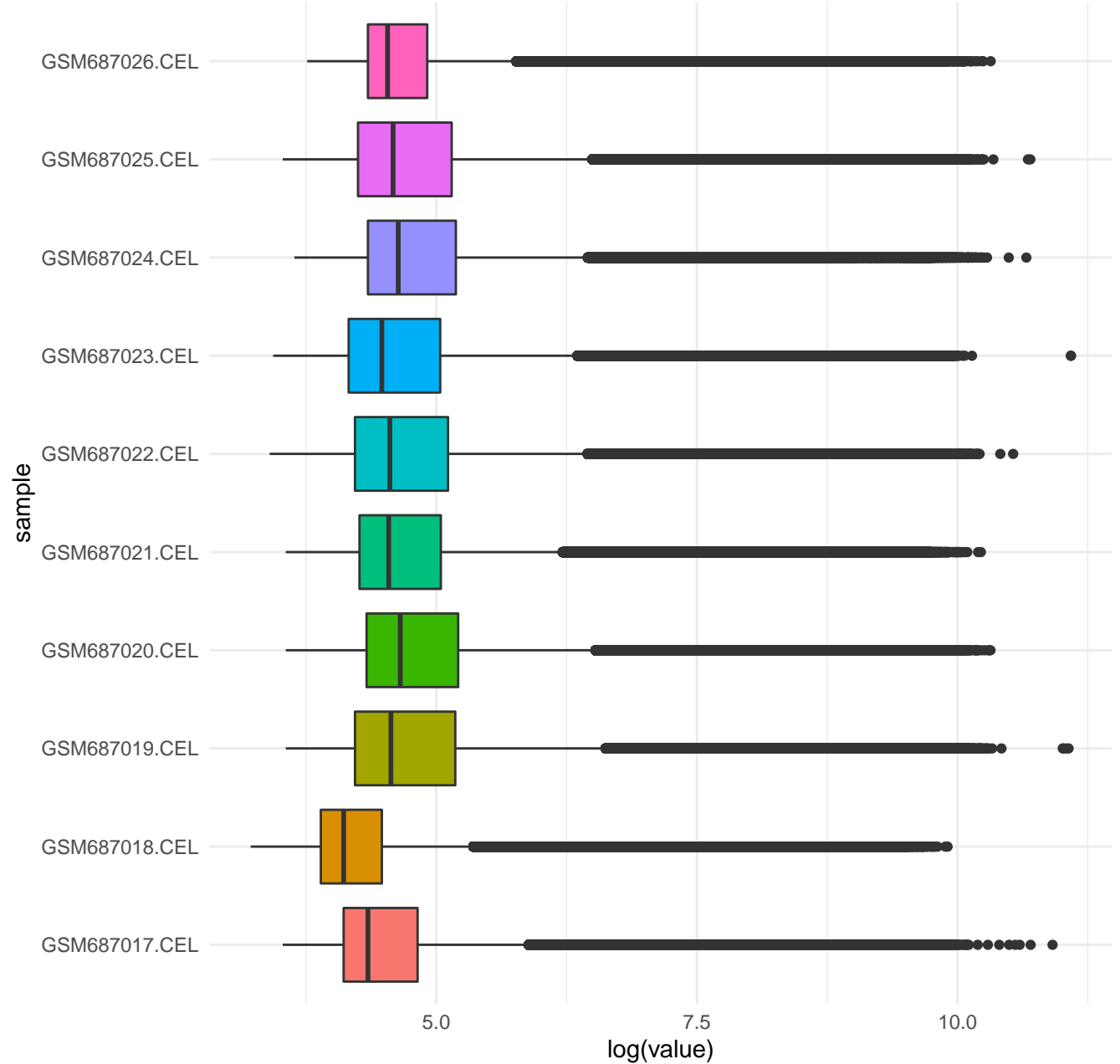
Breast cancer microarray data before normalization
