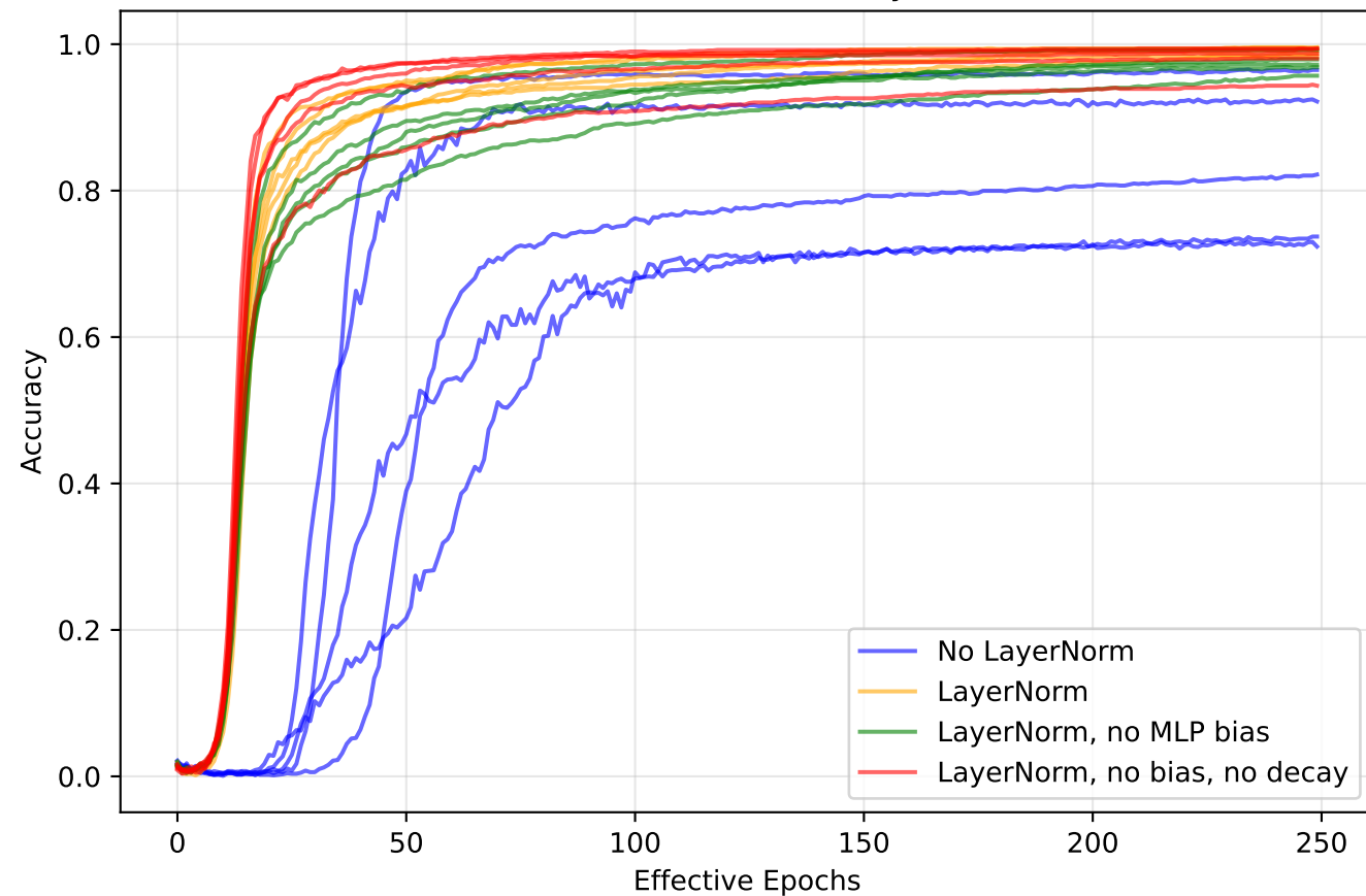
Validation Accuracy
