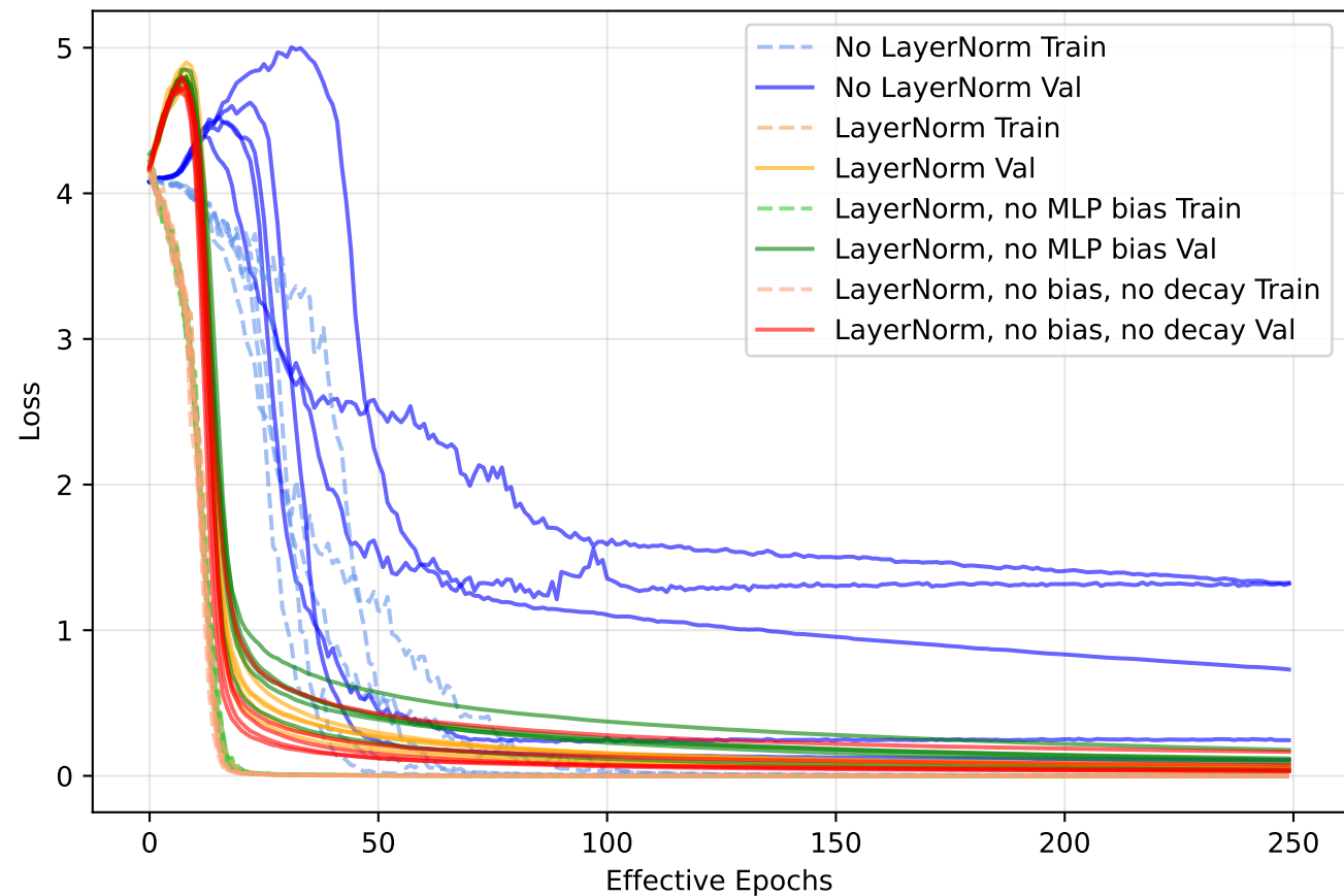
Loss
