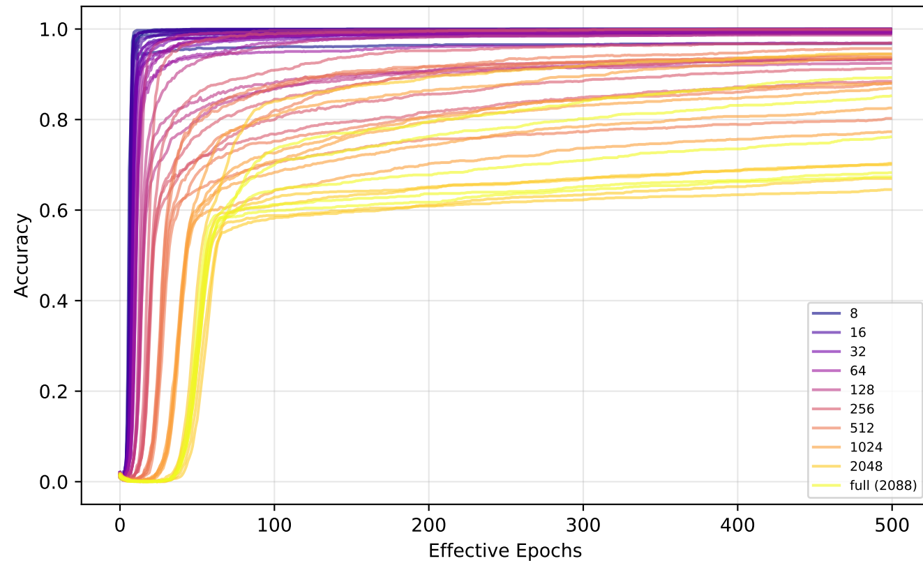
Validation Accuracy
