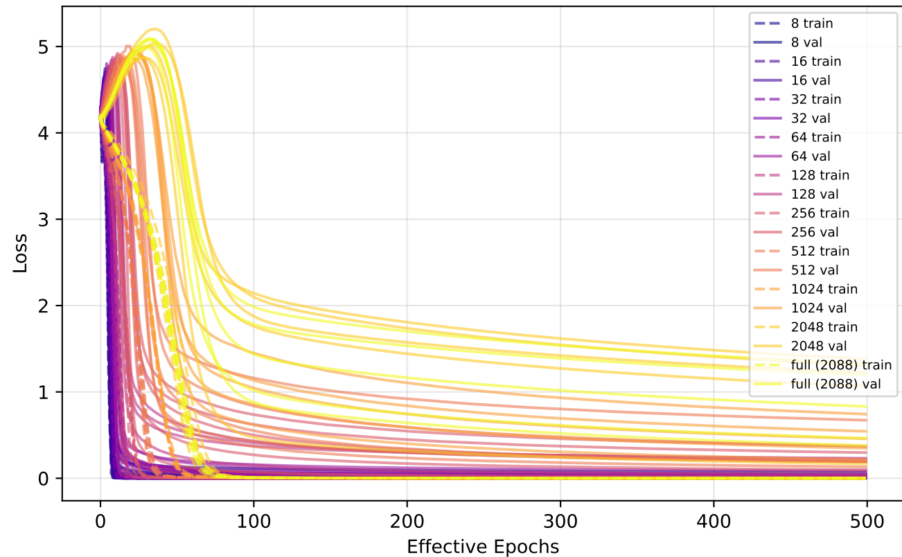
Loss
