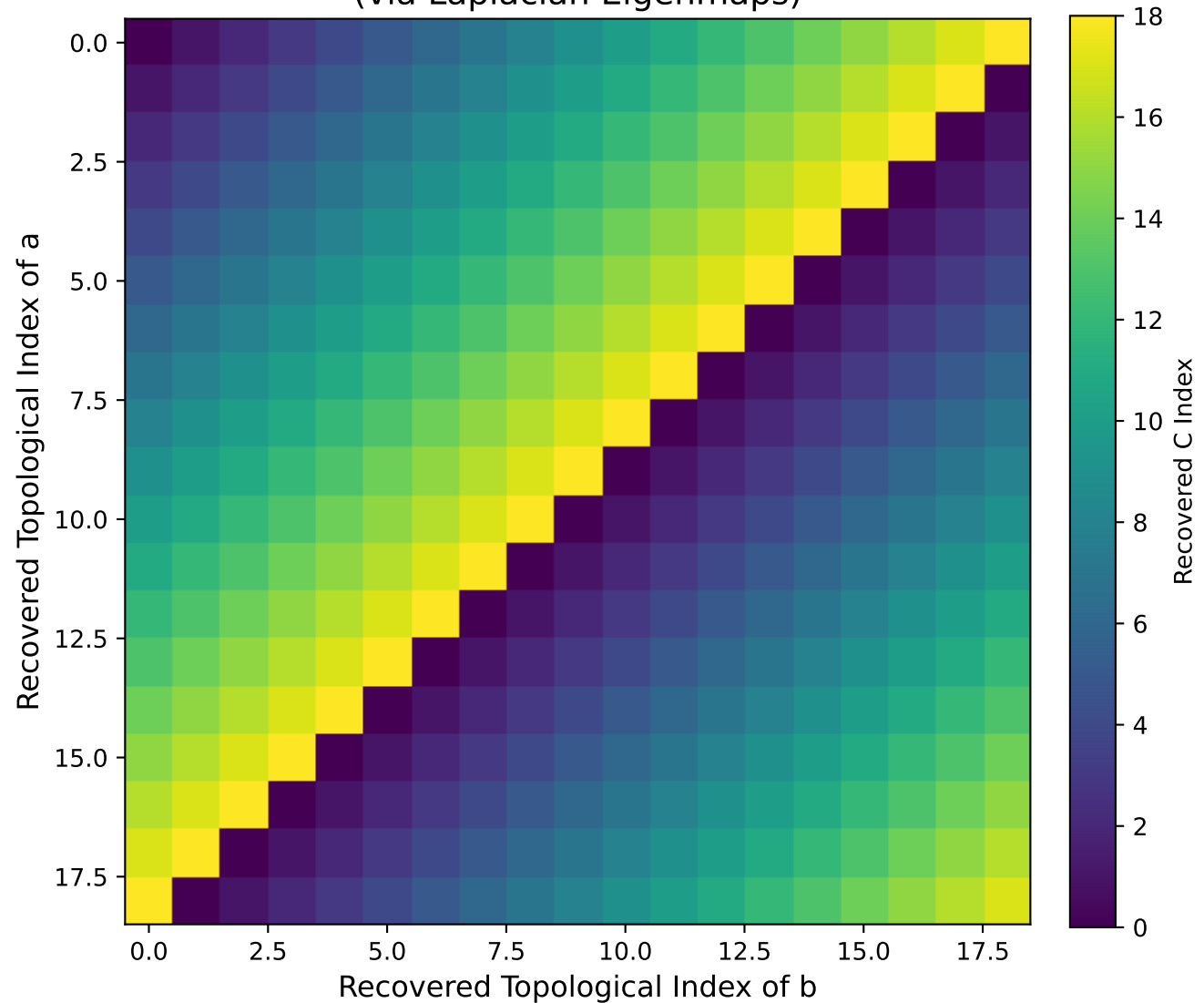
Recovered Structure (via Laplacian Eigenmaps)
