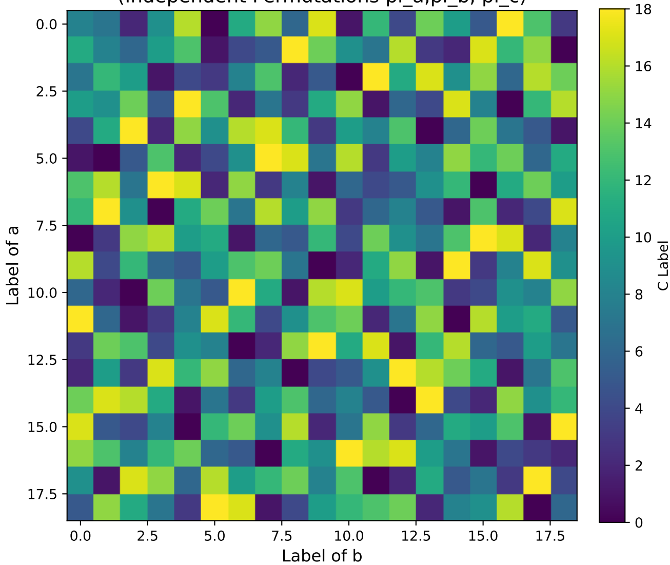
Observed C-Table (Independent Permutations \pi_a, \pi_b, \pi_c )
