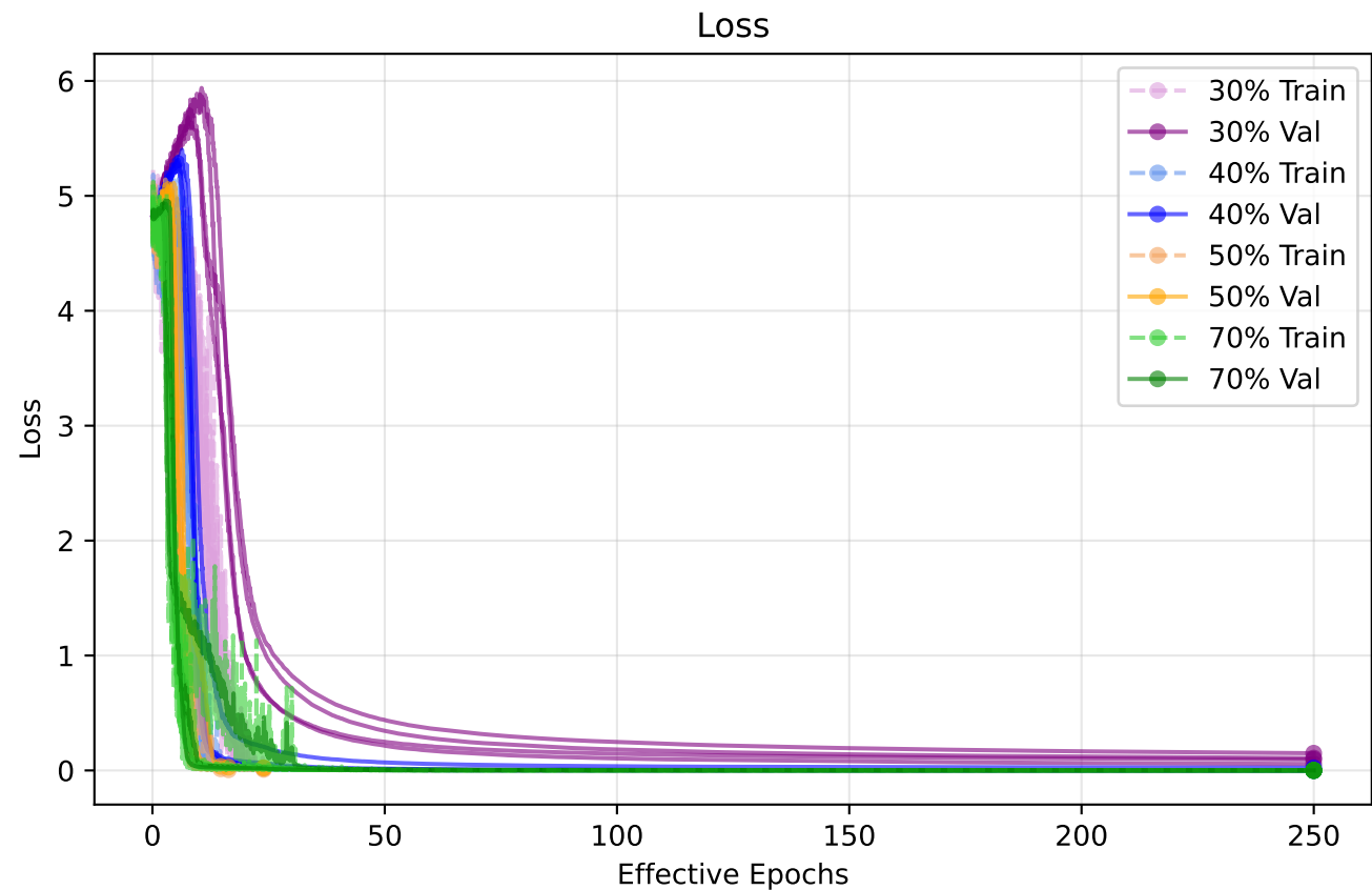
p=113, LayerNorm on, no MLP bias — varying train fraction
