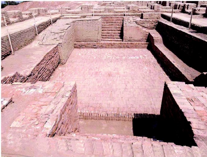
Fig. 20.7: Great Bath of Mohenjodaro (Dimensions 11.8x7metres)
