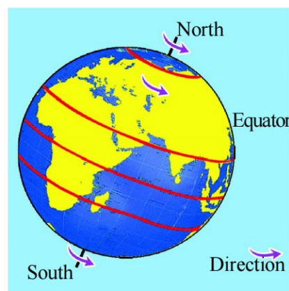
Fig. 2.3: Axis of rotation
