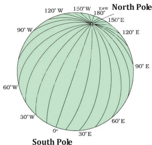
Fig. 2.5: Longitudes on the globe
