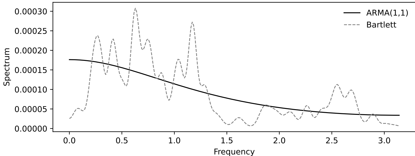
Figure 3. Spectral density of consumption growth
