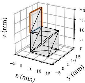
(c) non-manifold edge 3 boundary, 1 nonmanifold
