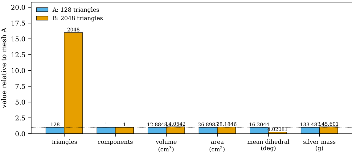
Measured comparison of two tessellations of one sphere (radius 15 mm)
