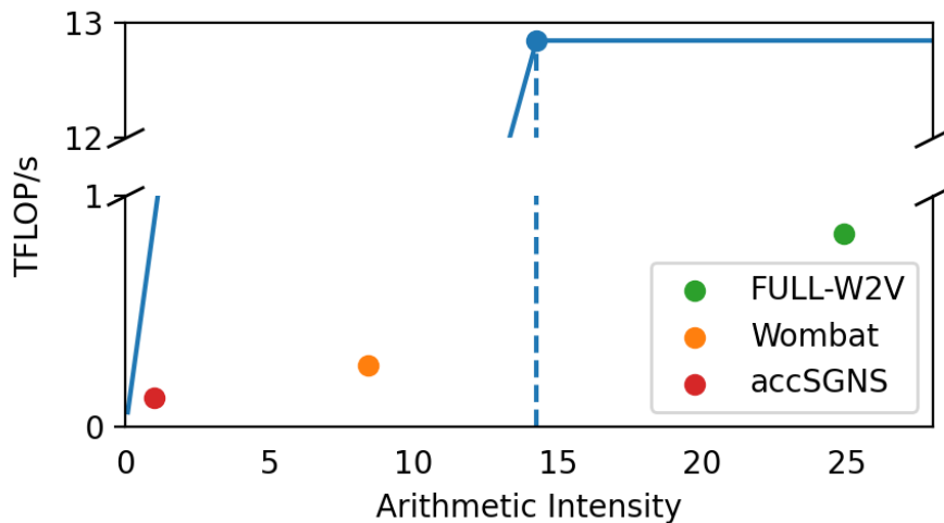
Figure 4.1: Roofline benchmarks for state-of-the-art kernels on a V100 GPU. The solid blue line is the roofline boundary, the dotted blue line marks the inflection point between memory-bound (left) and compute-bound (right). Previous work is memory-bound and exhibits poor overall throughput despite being data-intensive; our work, FULL-W2V, presents a significant improvement.
