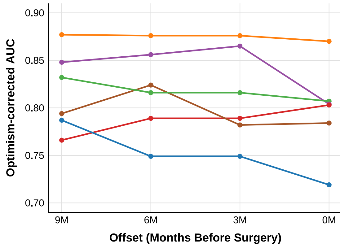
(B) XGBoost
