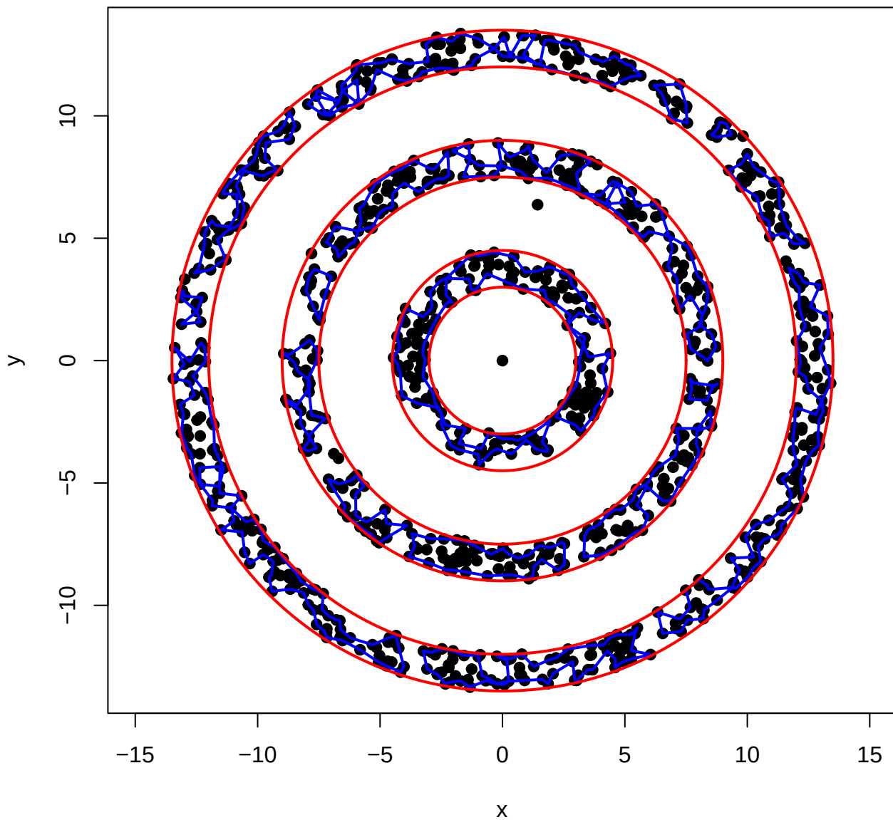
Alpha Shape Visualization – Alpha: 0.5 CL: 1 Noise: 0.001
