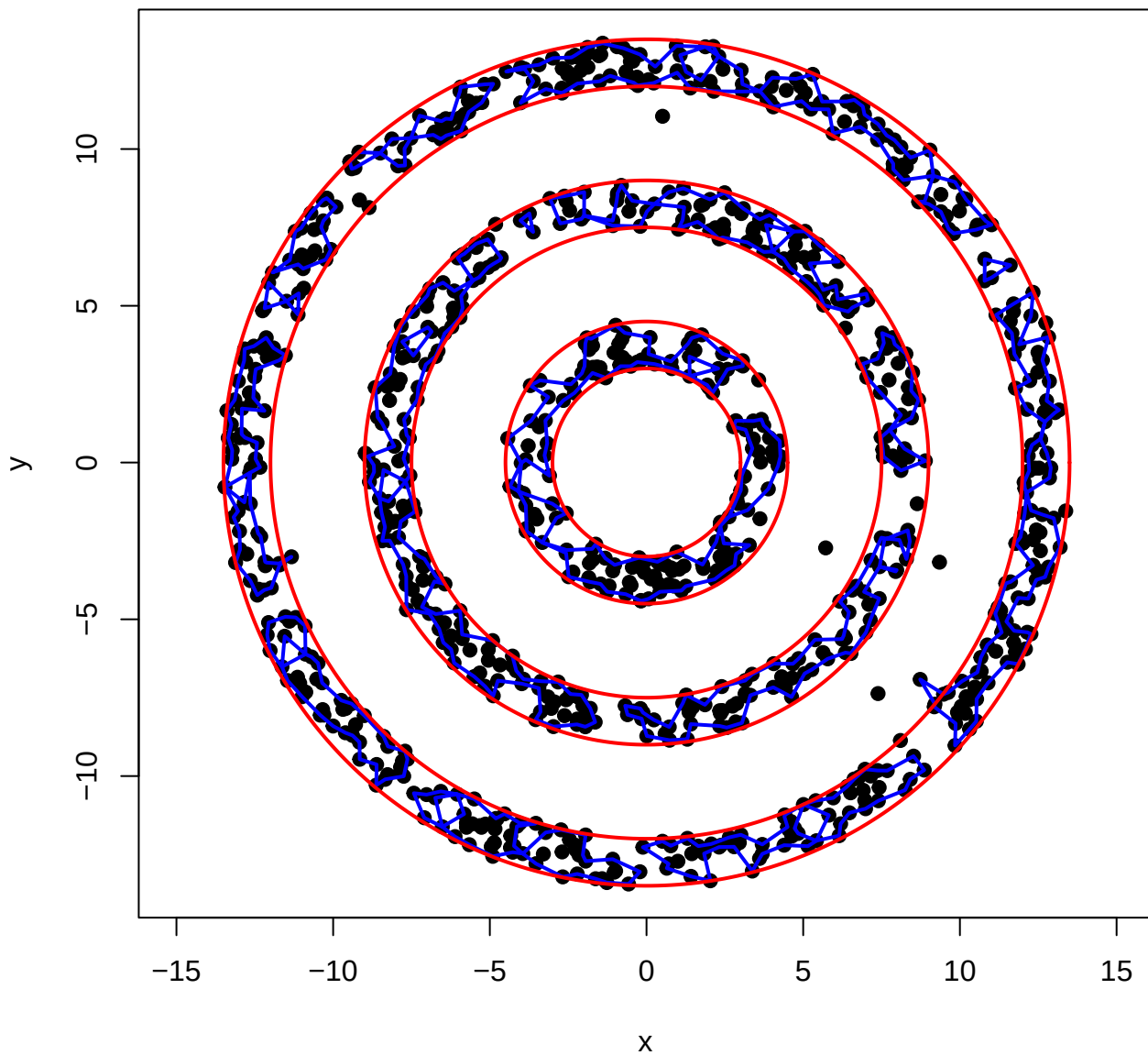
Alpha Shape Visualization – Alpha: 0.5 CL: 1 Noise: 0.01
