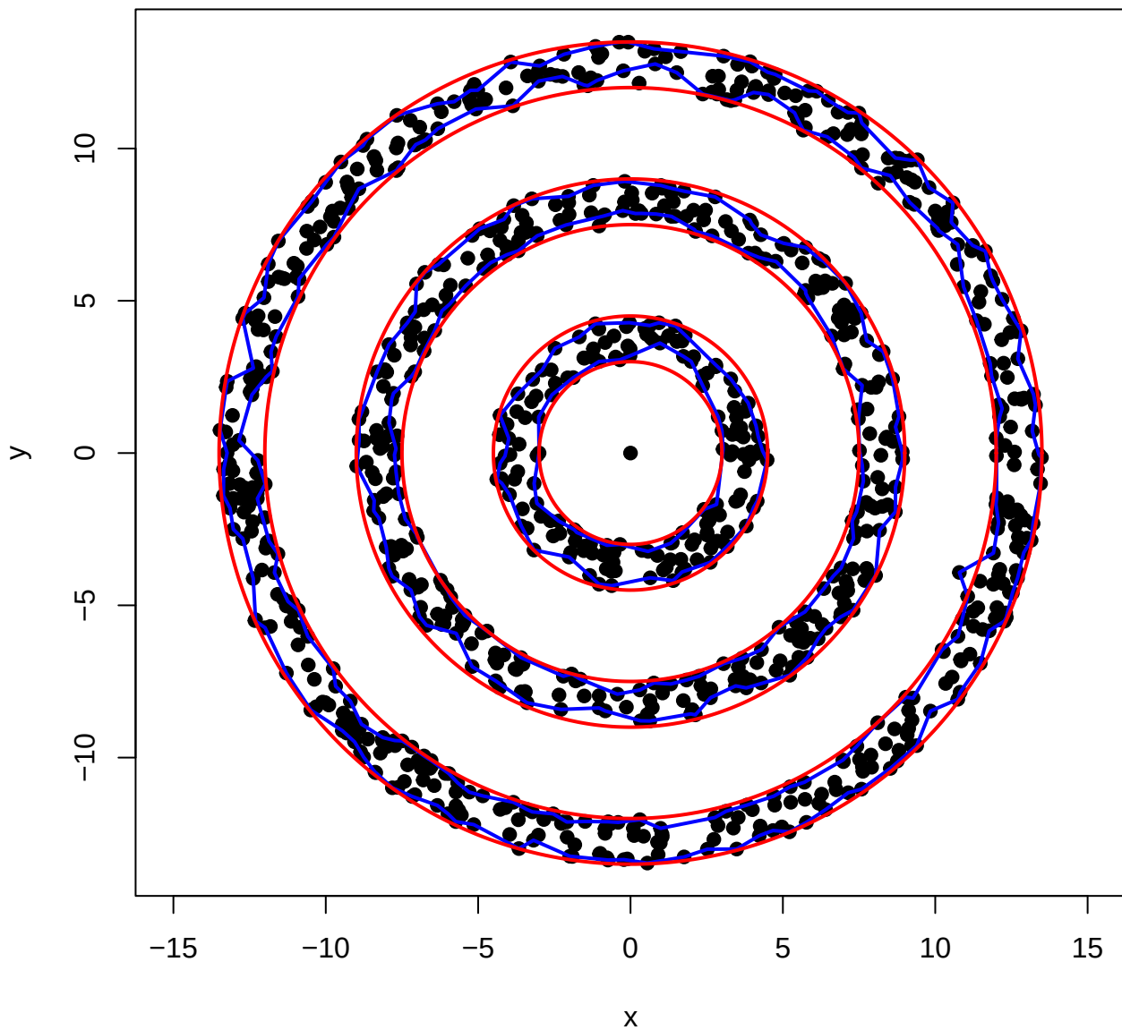
Alpha Shape Visualization – Alpha: 1 CL: 0.95 Noise: 0.001
