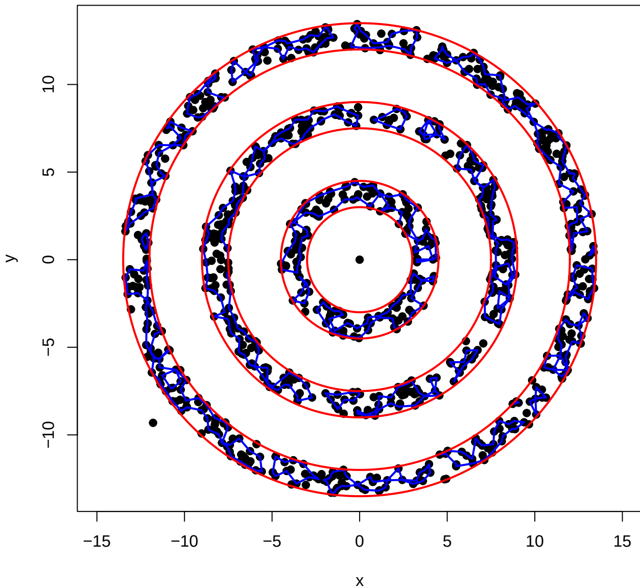
Alpha Shape Visualization – Alpha: 0.5 CL: 0.9 Noise: 0.001
