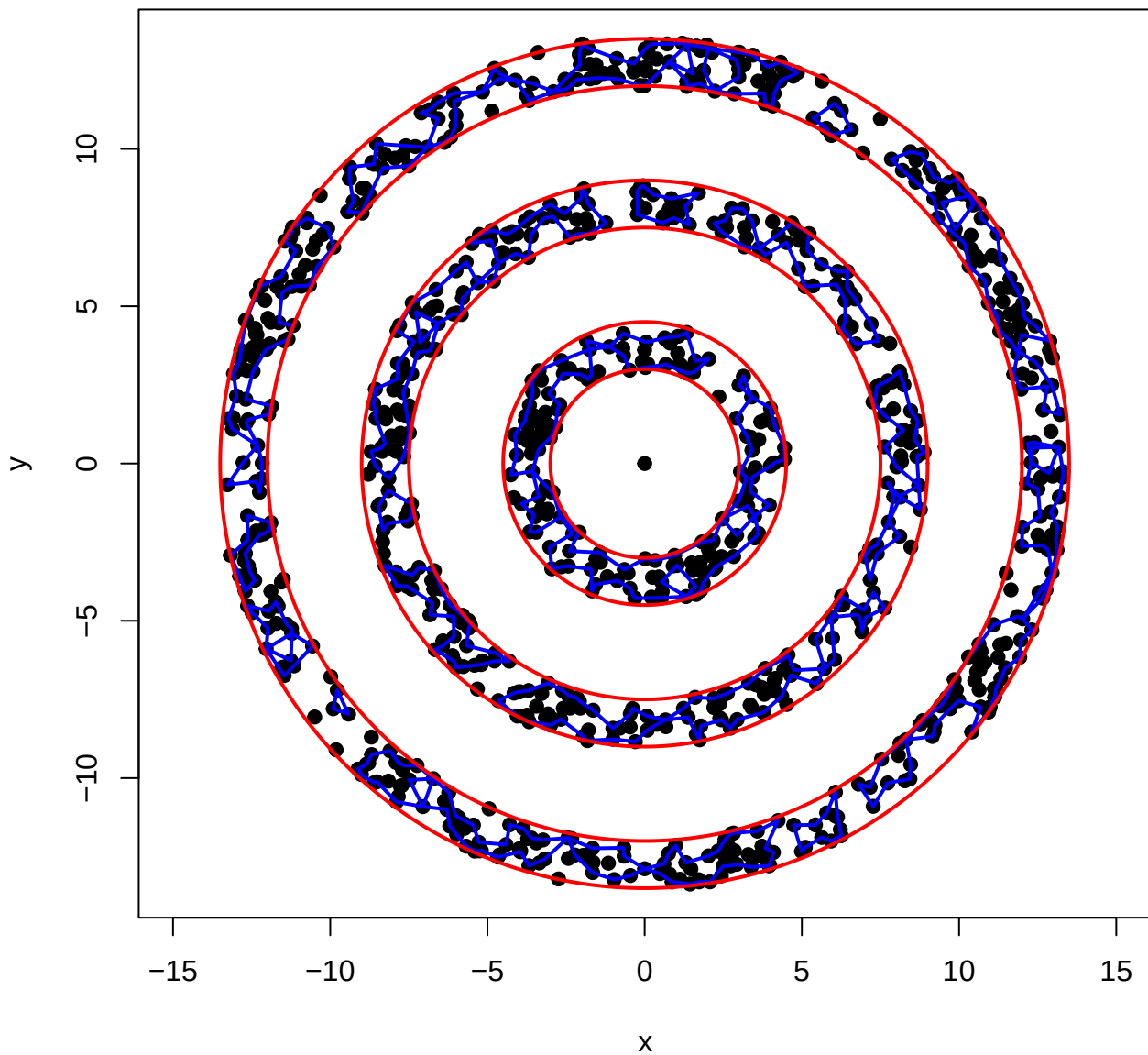
Alpha Shape Visualization – Alpha: 0.5 CL: 0.95 Noise: 0.001
