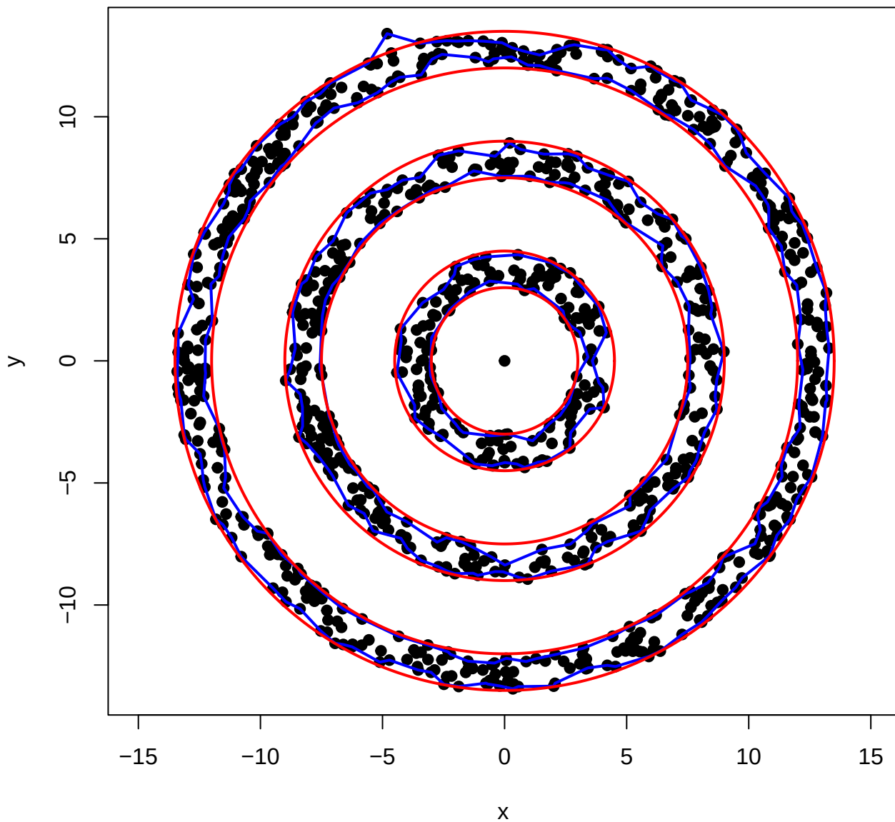
Alpha Shape Visualization – Alpha: 1 CL: 1 Noise: 0.001
