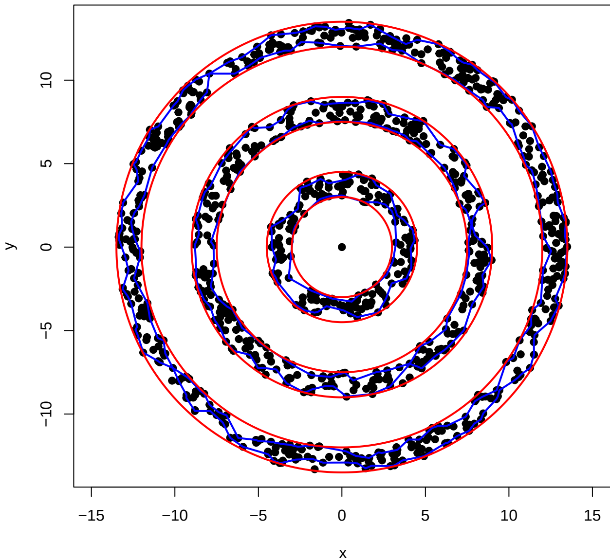
Alpha Shape Visualization – Alpha: 1 CL: 0.9 Noise: 0.001
