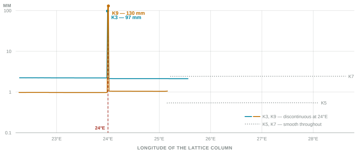
Figure 2. Second difference of AGKK's output along the lattice rows, per easting column, taken as the median across every row of the zone; logarithmic scale. K5 and K7 are flat across their full width (0.54 and 2.43 mm). K3 and K9 are equally flat except for a single spike reaching 97 and 130 mm — exactly at 24°E.
