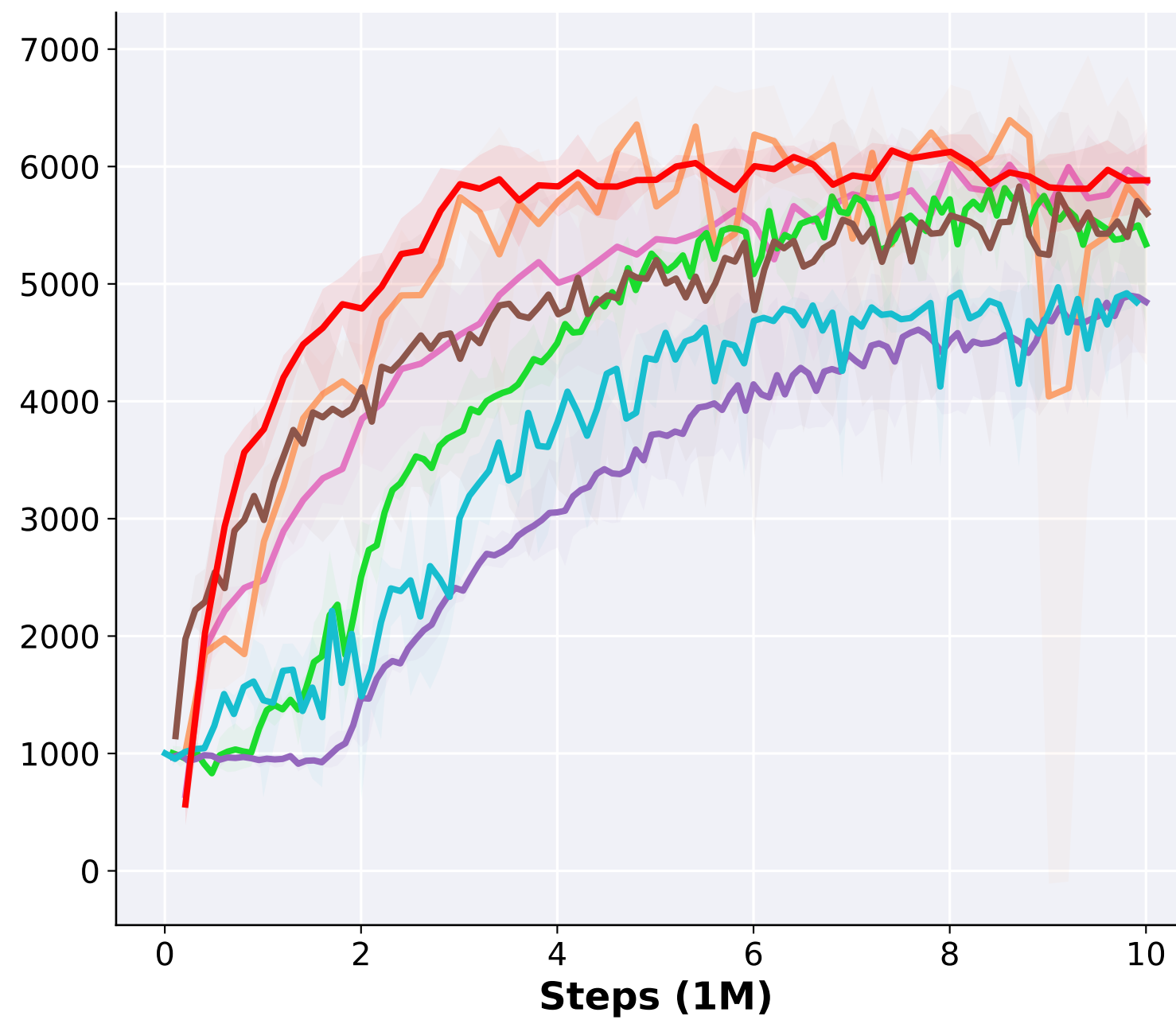
(e) Ant 8x1
