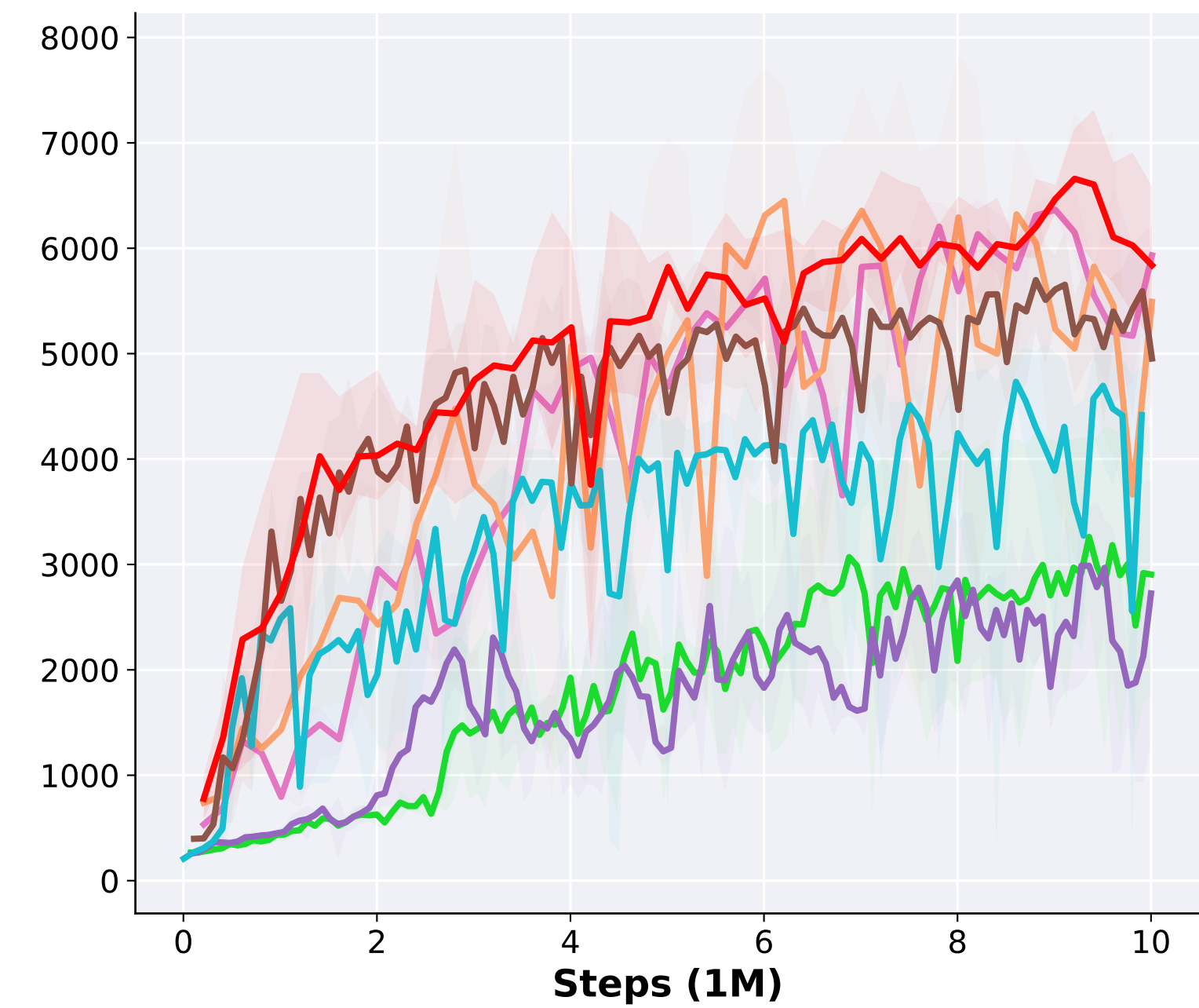
(c) Walker2d 2x3
