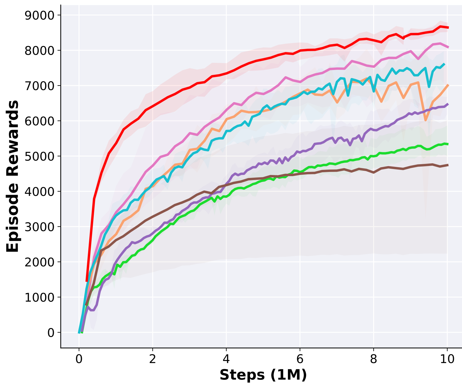
(a) HalfCheetah 3x2
