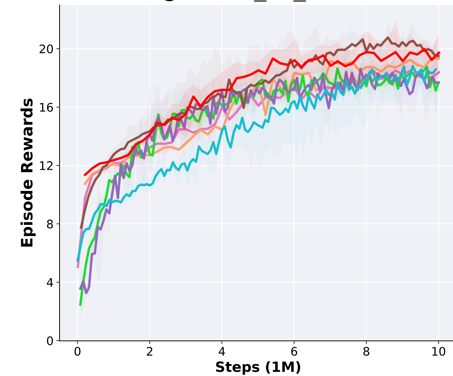
(g) 3s5z_vs_3s6z
