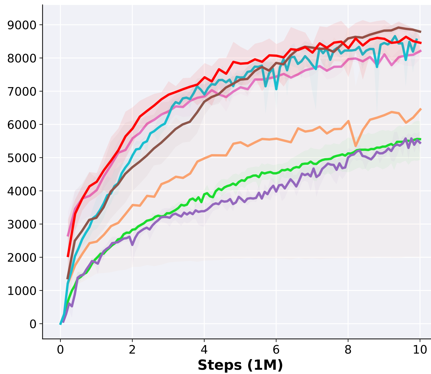
(b) HalfCheetah 6x1
