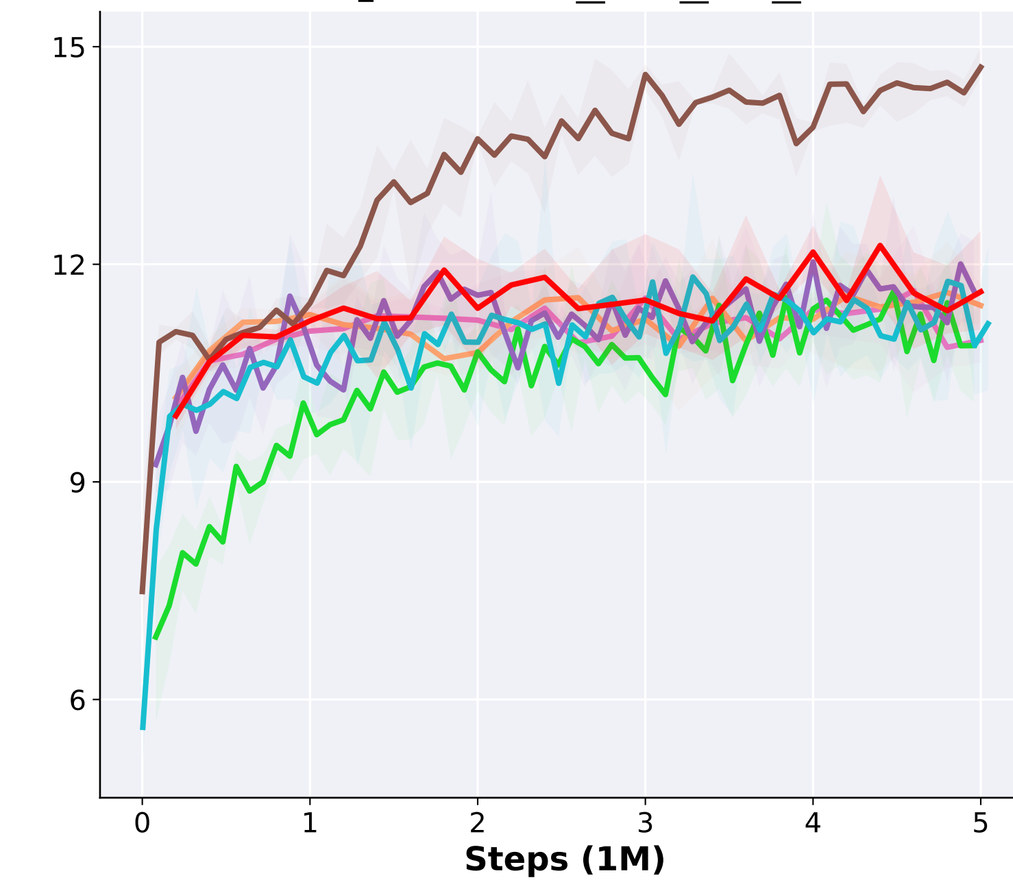
(h) protoss_10_vs_11
