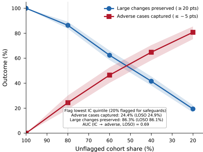
B Illustrative enrichment: flag by IC quintile
