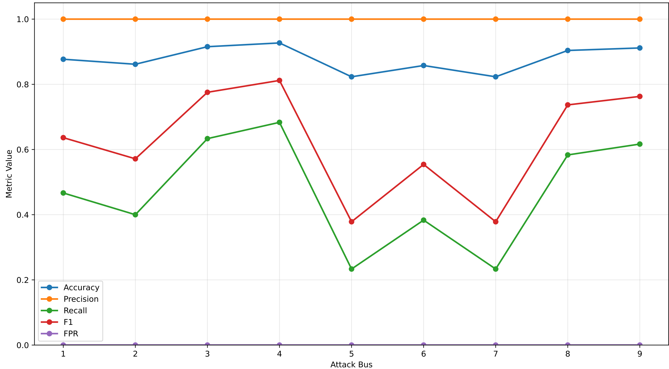
IEEE-9 Bus Attack Detection Performance
