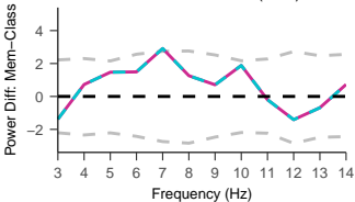
Mem. vs Class. HR (FFT)
