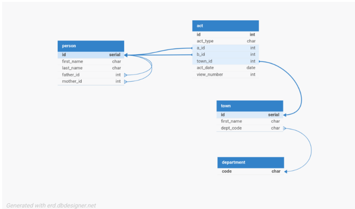
Figure 1: Database Relation Schema
