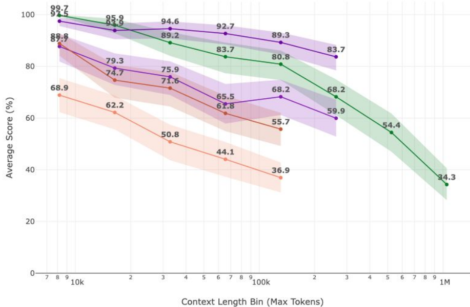
OpenAI-MRCR: Top Performers (4-Needle)
