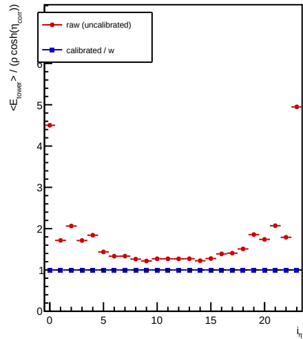
hcalout
