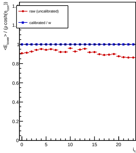
cemc
