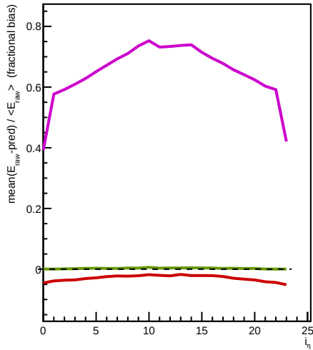
hcalin (full-tower stats)
