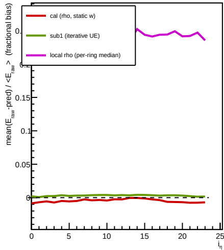
cemc (full-tower stats)
