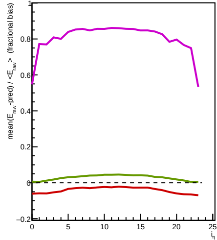
hcalout (full-tower stats)
