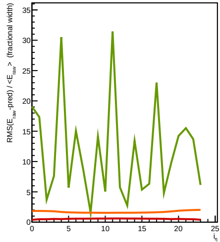
hcalout
