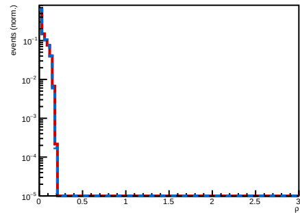
\rho HCALOUT
