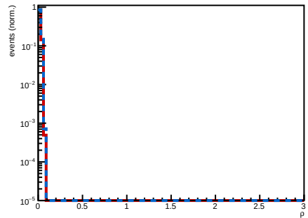
\rho HCALIN
