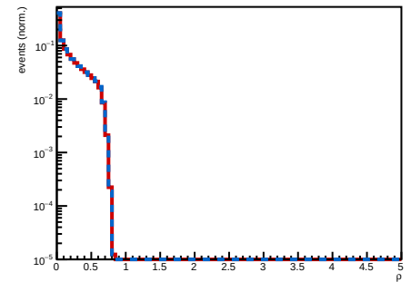
\rho CEMC
