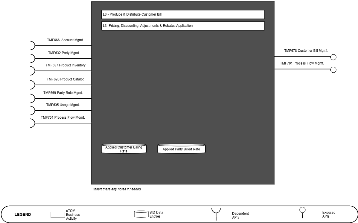
TMFC031: Bill Calculation
