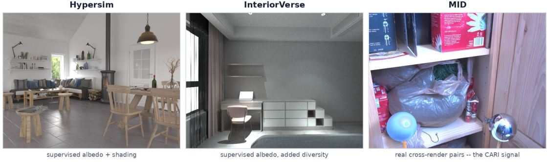
Figure 4.2: Hypersim and InteriorVerse are both synthetic and both supply supervised albedo; MID is real and is the only source of the paired cross-illuminant observations CARI is trained on. No single dataset provides everything the model needs.
