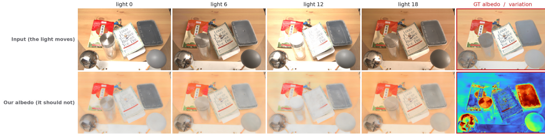
Figure 5.9: Qualitative albedo constancy on one MID scene. The upper row shows four inputs and the pseudo-ground-truth albedo; the lower row shows the corresponding predictions and a per-pixel variation heatmap (red = the prediction changes with the light). The predicted material colours stay stable across illuminants, yielding cool (blue) CoV maps on the flat surfaces where the light changes most.
