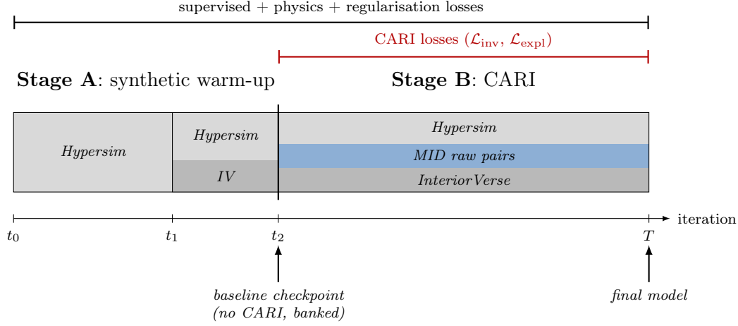
Figure 4.5: Two-stage training schedule. Stage A establishes the supervised baseline on synthetic data ( Hypersim , later joined by InteriorVerse ). Stage B resumes from the Stage-A checkpoint and adds MID raw pairs with the CARI losses, keeping the synthetic majority as the absolute-colour anchor. The Stage-A checkpoint doubles as the no-CARI baseline in the ablation study (Sect. 5.6).
