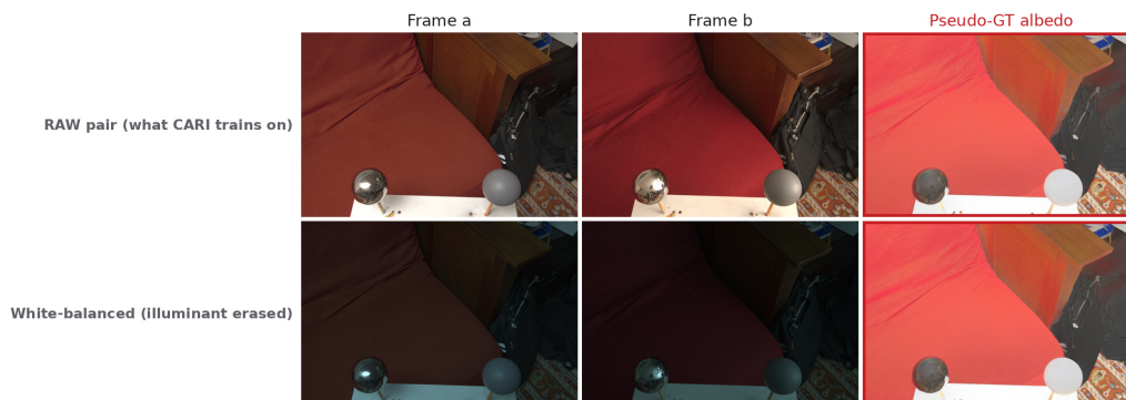
Figure 4.2: MID preprocessing used during training; this is a data-loading diagram, not an evaluation protocol. The supervised path uses a white-balanced primary frame and the dataset pseudo-ground-truth albedo to anchor absolute material colour on real photographs. The CARI path keeps two aligned frames raw, without white balance, and masks pixels that are clipped or too dark in either exposure before applying the cross-render losses. This split keeps the albedo target stable while preserving the illuminant chromaticity change that CARI needs as supervision.
