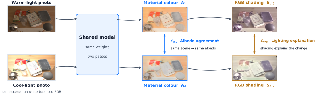
Figure 3.4: CARI applies only during training. The same shared-weight model runs twice, once per illuminant, on two real photographs of one MID scene; the resulting albedo predictions \mathbf{A}_1 and \mathbf{A}_2 are pushed together by \mathcal{L}_{inv} (Eq. (3.7)). Inference sees only one branch of this diagram: a single image through a single forward pass, with no pairing and no extra cost.
