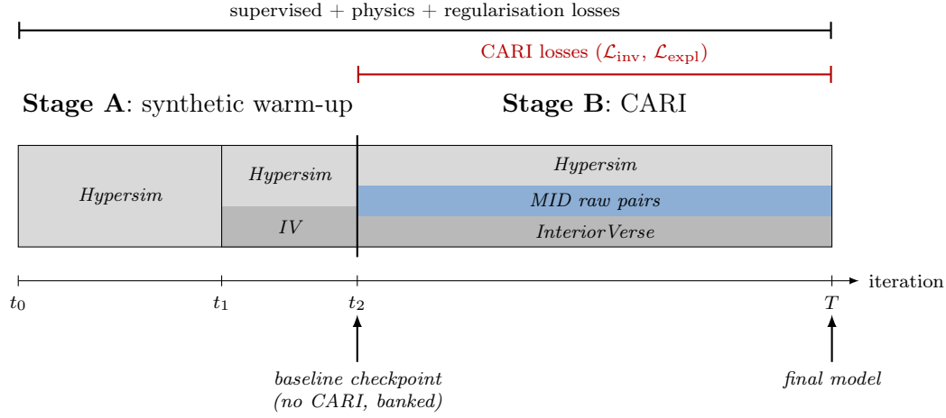
Figure 4.4: Two-stage training schedule. Stage A establishes the supervised baseline on synthetic data (Hypersim, later joined by InteriorVerse). Stage B resumes from the Stage-A checkpoint and adds MID raw pairs with the CARI losses, keeping the synthetic majority as the absolute-colour anchor. The Stage-A checkpoint doubles as the no-CARI baseline in the ablation study (Sect. 5.6).
