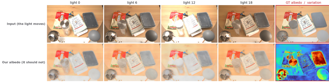
Figure 5.8: Qualitative albedo stability on one MID scene. The upper row shows four inputs and the pseudo-ground-truth albedo; the lower row shows the corresponding predictions and a per-pixel coefficient-of-variation map of predicted luminance (red = the prediction changes with the light). The map stays cool over the table and most of the matte packaging, and turns red on the plastic tray, the glass jar and the mirror sphere, surfaces an albedo-shading product cannot represent; the book cover also washes out under the brightest flash (light 12).
